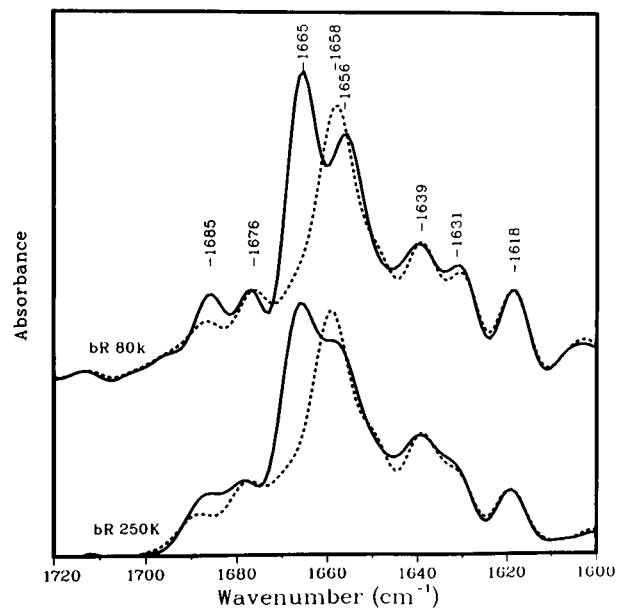
FIGURE 5 Amide I region for hydrated PM at 80 K (top) and 250 K (bottom) with parallel (solid) and perpendicular (dashed) polarization after Fourier self-deconvolution (half width = 16 cm^{-1} , k = 2.0 ).
