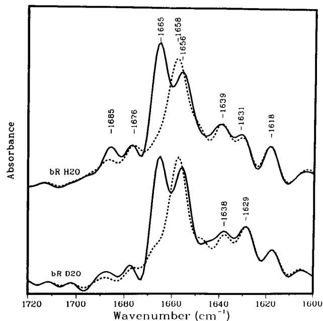
FIGURE 6 Amide I region for hydrated (A) and deuterated after 48 h (B) PM recorded at 80 K with parallel (solid) and perpendicular (dashed) polarization. Deconvolution parameters are as in Fig. 5.
