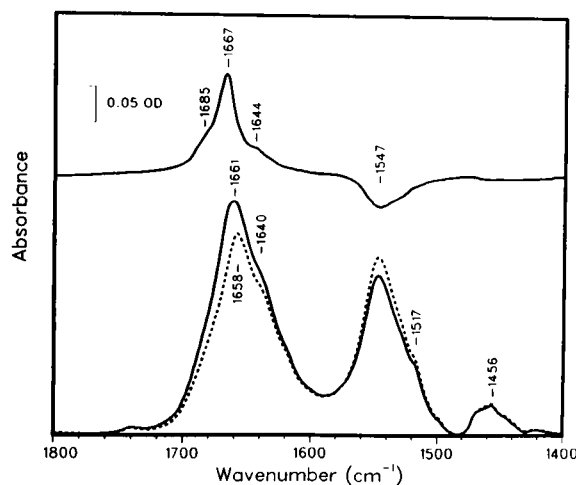
FIGURE 1 Polarized FTIR spectra of hydrated purple membrane at 280 K. (Bottom) Spectra taken with incident beam polarized perpendicular, A_{\perp} , (dashed line) and parallel, A_{\parallel} , (solid line) to the plane of incidence. (Top) A_{\parallel} - A_{\perp} .
